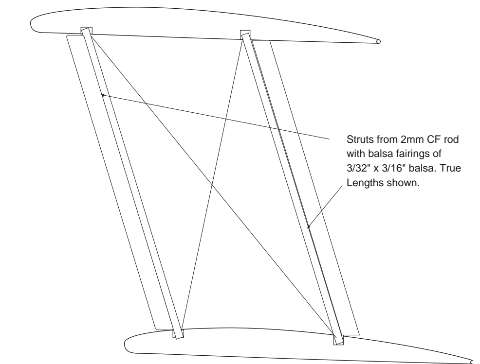
Interplane struts and optional rigging
