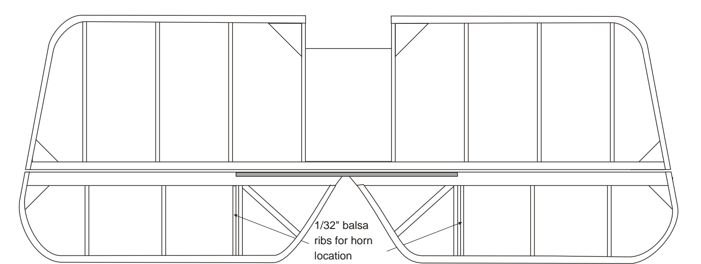
Tailplane from 1/16" strip as shown, outer curve 3x 1/64" x 1/16" ply laminated, 1.5mm CF rod joiner..
